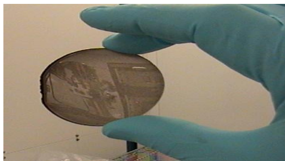
Figure 2. Free standing polycrystalline diamond, ~50 mm diameter and ~230 \mu\text{m} thick.
