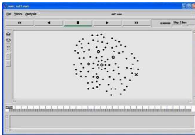
Figure 6. Node Creation
