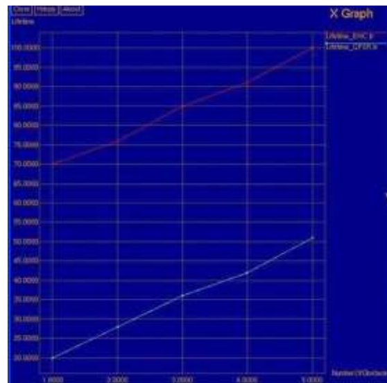
Figure 16. Lifetimes of EHC and GPSR
