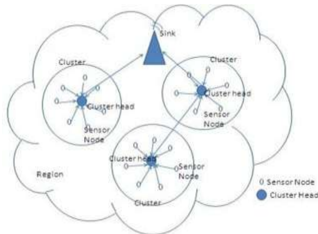
Figure 2. Clustered Networks
