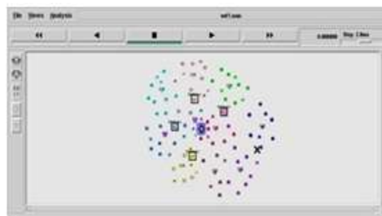
Figure 7. Cluster Formations
