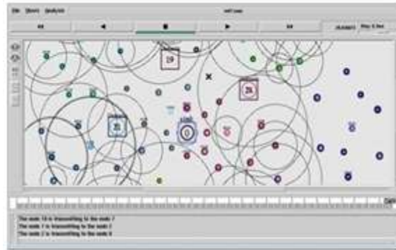
Figure 11. DataTransfer
