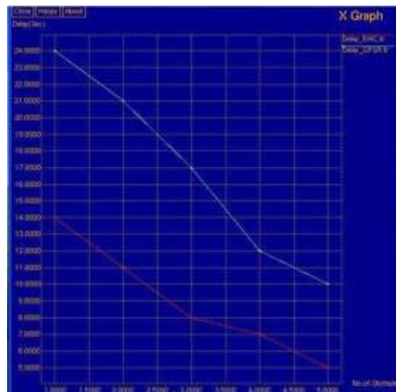
Figure 15. Comparison of Delay between EHC and GPSR
