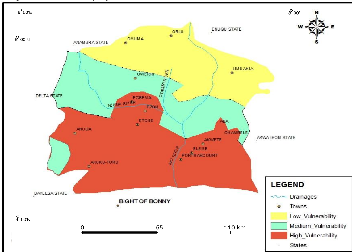
Figure 2: Groundwater Vulnerability Map of part of Eastern Niger Delta
