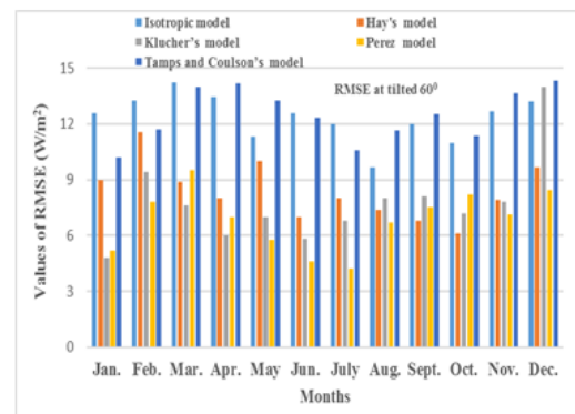
Figure (22): The values of RMSE at tilted 60° (W/m 2 )
