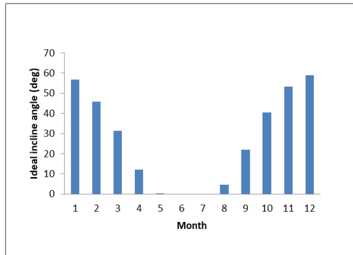
Figure (11): Monthly variation of ideal incline angle for a south-facing flat surface in Jeddah
